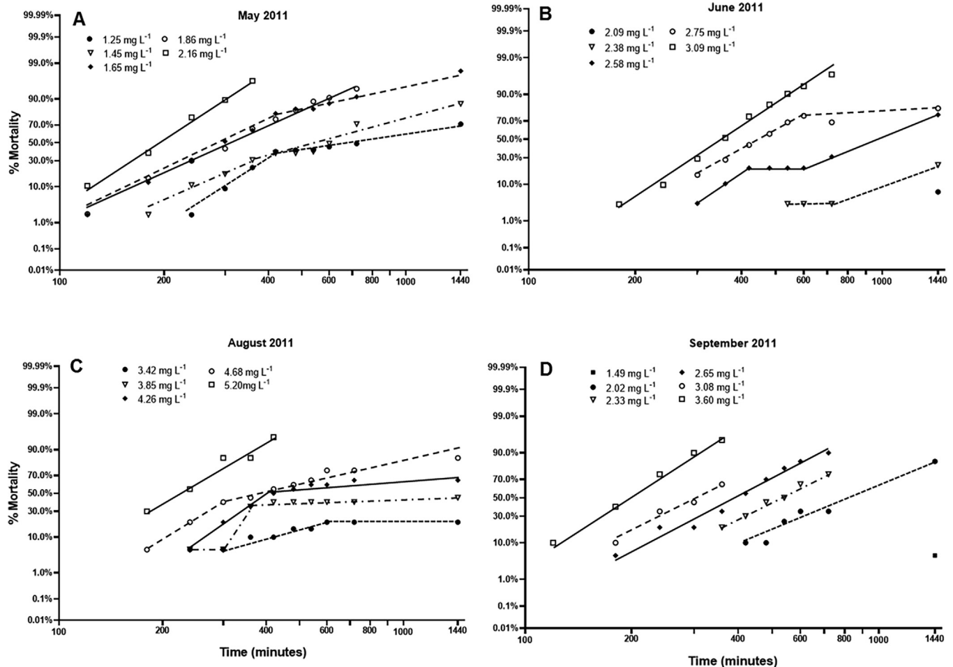
Fig. 3. Relationship between season and time to lethality during TFM exposure. Time versus lethality relationship in larval sea lamprey exposed to different concentrations of TFM captured from Deer Creek, MI, in (A) May, (B) June, (C) August and (D) September 2011. The exposure concentrations of TFM used for this analysis were those used to determine the 12-h LC 50 and LC 99.9 in Fig. 2. Data depicted as % mortality, on a probit scale, plotted against time (24 h) on a logarithmic scale. Lines of best fit were determined by non-linear regression (Prism 8.03, Graphpad Software, La Jolla, CA), and used to determine the corresponding LT 50 values ( \pm 95\% CI) values (Table 2). N = 53–57 per test concentration in May, N = 28–31 in June, and N = 20 in August and September.
