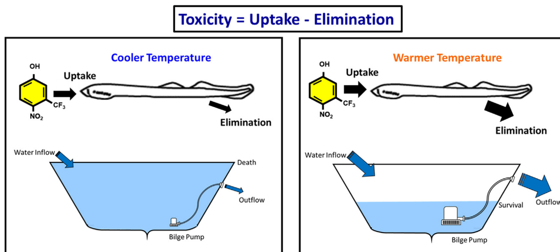
Fig. 8. Proposed working model of TFM tolerance in larval sea lamprey at cool and warm temperatures. Toxicity is the difference between rates of toxicant (TFM) uptake minus elimination. In sea lamprey, TFM is likely detoxified in the liver, which results in the generation of the less toxic metabolite TFM-sulphate, and possibly small amounts of TFM-glucuronide (Bussy et al. 2018a, b), which are more water soluble and then eliminated. In cooler waters, if rates of TFM uptake are greater than detoxification-elimination, TFM will accumulate to toxic levels causing death. Despite higher rates of TFM uptake at warmer temperatures, it is predicted that rates of TFM elimination are also increased, exceeding the rates of TFM uptake, resulting in less TFM accumulation and greater survival. In each case the liver can be thought of as a bilge pump on a boat, which removes the water (TFM) more efficiently at warmer temperatures.
