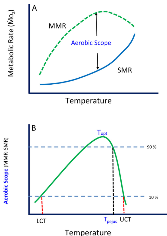
Fig. 7. Aerobic Scope and Thermal Performance Curves. (A) Aerobic scope is measured by first measuring standard metabolic rate (SMR) in resting, post-absorptive animals, followed by measurements of maximal metabolic rate (MMR), usually by determining M_{O_2} following exhaustive chasing. Aerobic scope, the difference between MMR - SMR , is then calculated at different temperatures. (B) The measurements of aerobic scope are then plotted against temperature, to generate thermal performance curves, which are fitted by non-linear regression or a quadratic equation as appropriate. T_{opt} : Optimum temperature for aerobic scope (performance). See text for further details.
