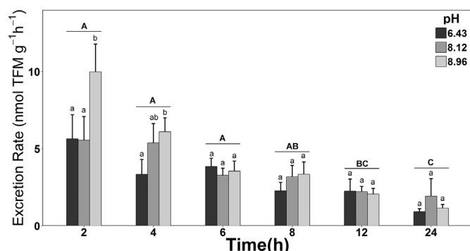
Fig. 3. Effects of pH on excretion rates of 3-trifluoromethyl-4-nitrophenol. Changes in excretion rates of 3-trifluoromethyl-4-nitrophenol (TFM) by larval sea lamprey at different pHs (low, moderate, and high pH) when injected with 85 nmol TFM g -1 . Data is presented as the mean ± SEM, (N = 8 per treatment). Statistically significant differences between time periods are denoted by upper case letters while the excretion rates within each group are denoted by lower case letters at each time period. Rates observed at pH low, moderate, and high pH are presented by dark bars, grey bars, and light grey bars, respectively.
