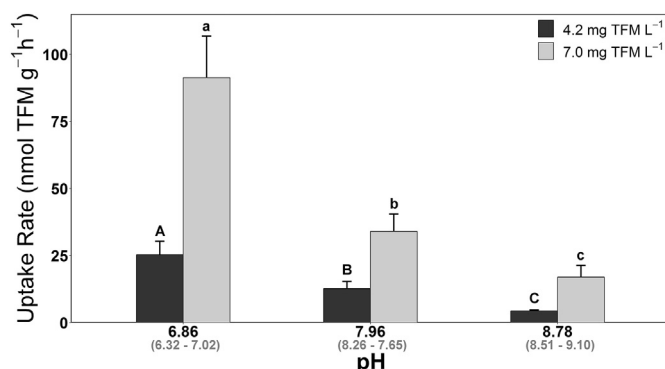
Fig. 2. Effects of pH on the rate of 3-trifluoromethyl-4-nitrophenol uptake. Changes in the TFM uptake rates of larval sea lamprey during exposure to 3-trifluoromethyl-4-nitrophenol (TFM) at 4.2 \text{ mg TFM L}^{-1} for 3 h (black bars) and 7.0 \text{ mg TFM L}^{-1} , for 1 h (light grey bars) at three different pHs (low, moderate, and high pH). Overall average pH between the two experiments for low, moderate, and high pH is on the x axis with the range indicated underneath. Data are presented as the mean \pm SEM ( N = 9\text{--}12 fish at each pH). Statistically significant differences between the rates of TFM uptake or accumulation at each pH are denoted by upper case and lower case letters during exposure to 4.2 \text{ mg TFM L}^{-1} and 7.0 \text{ mg TFM L}^{-1} , respectively. The average pH between the two experiments is on the x-axis (black text) with the range of pH during the two experiments in parenthesis is underneath (light grey text).
